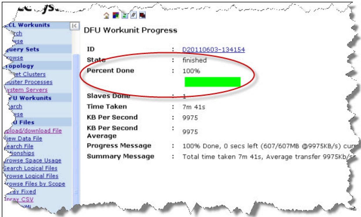
Figure 6. Workunit Progress
