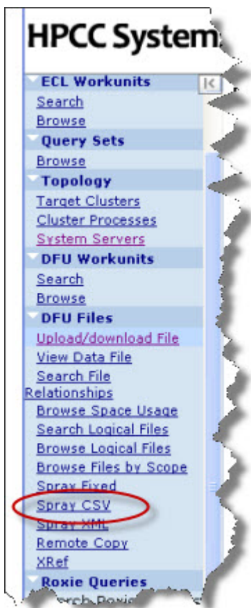
Figure 3. Spray CSV
