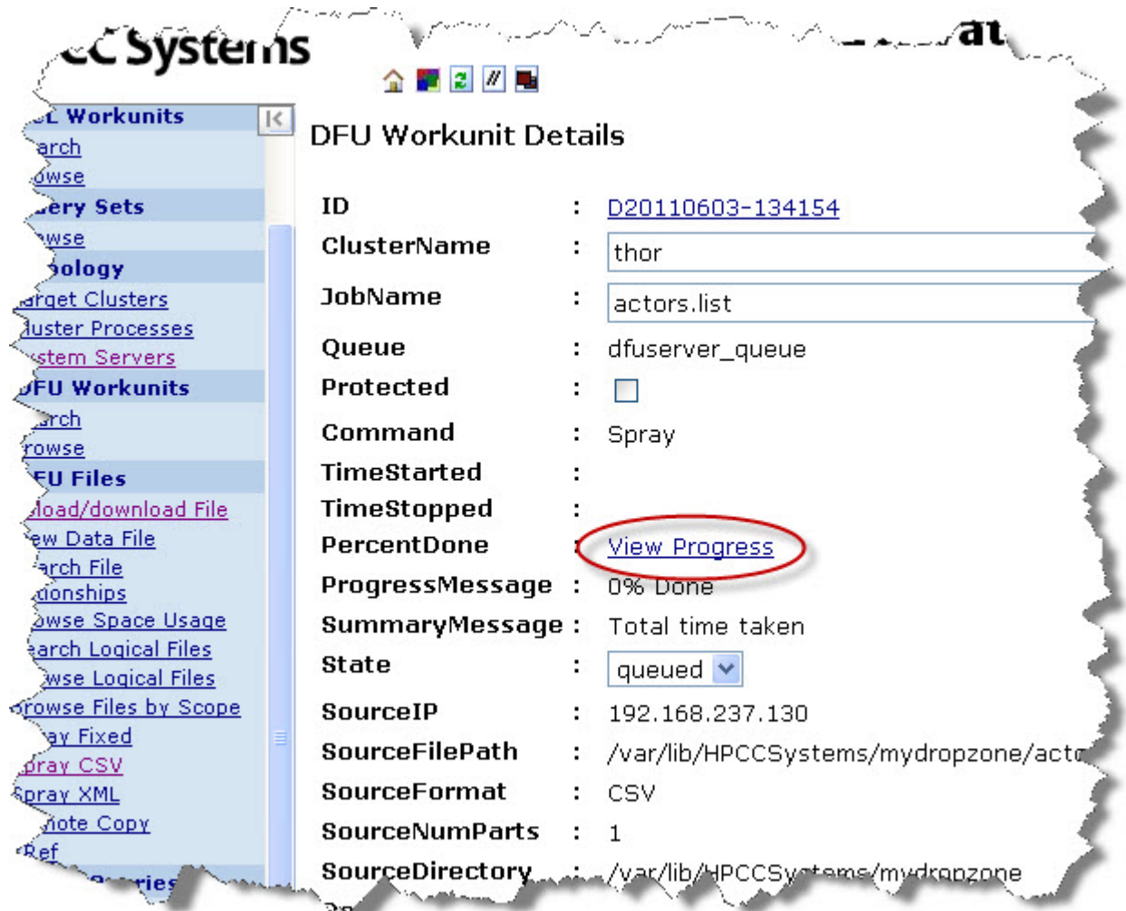
Figure 5. View Progress
