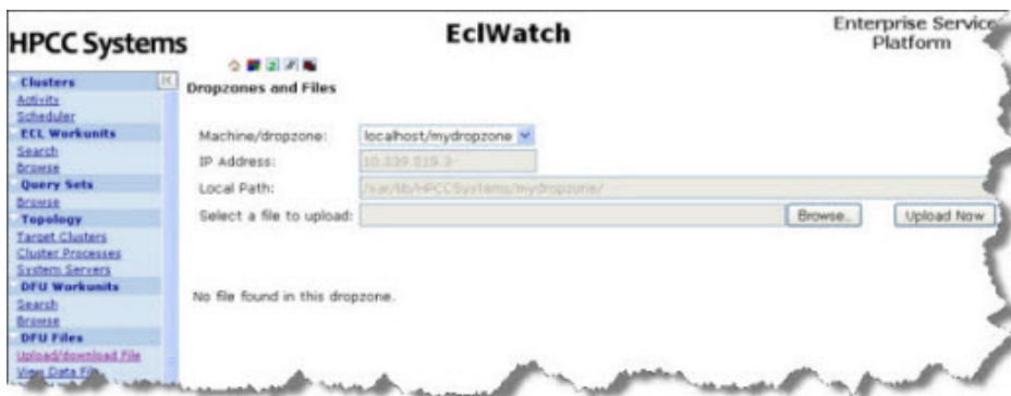
Figure 31. Dropzones
