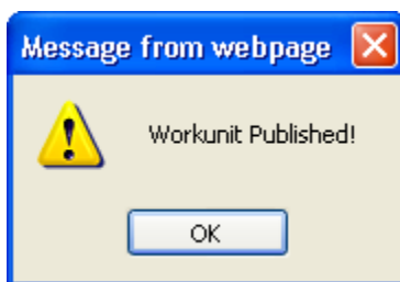
Figure 27. Workunit Published
