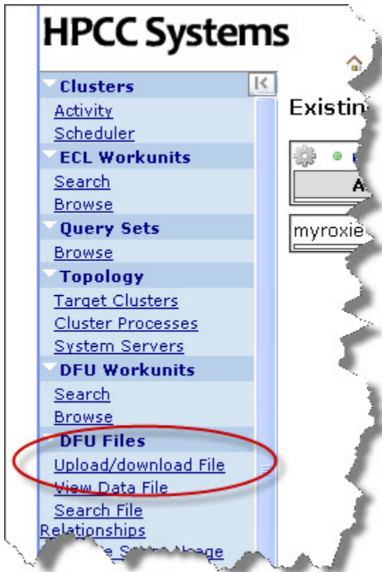
Figure 15. Upload/download
