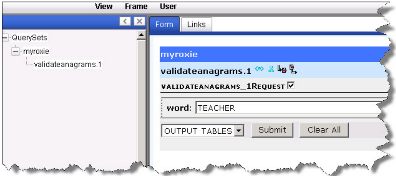
Figure 28. RoxieECL
