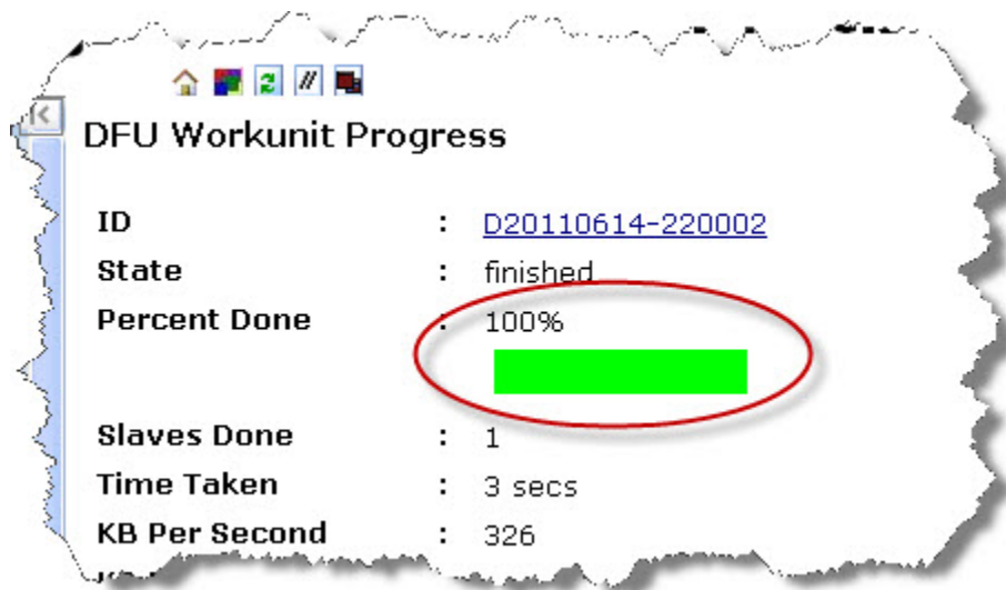
Figure 20. Workunit Progress
