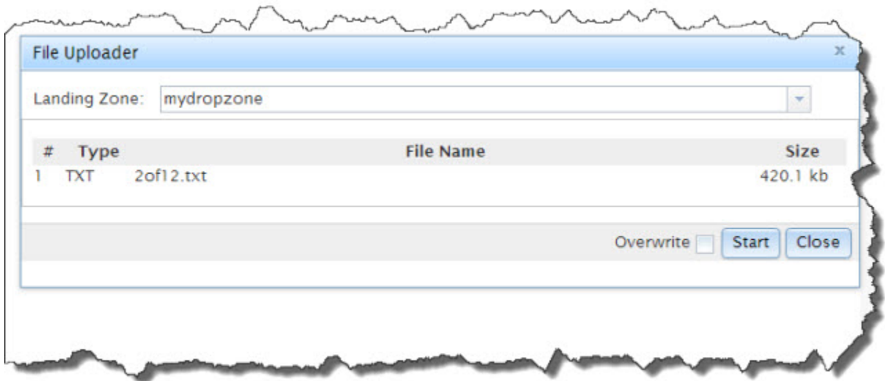
Figure 22. File Uploader
