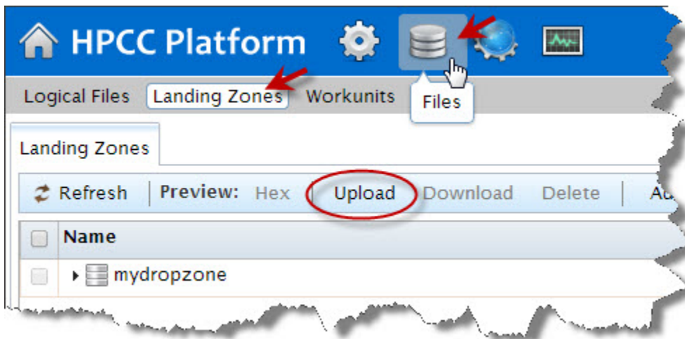
Figure 32. Upload/download
