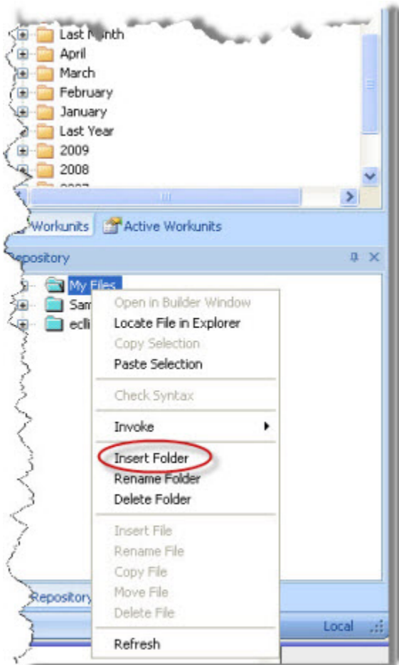
Figure 24. Insert Folder
