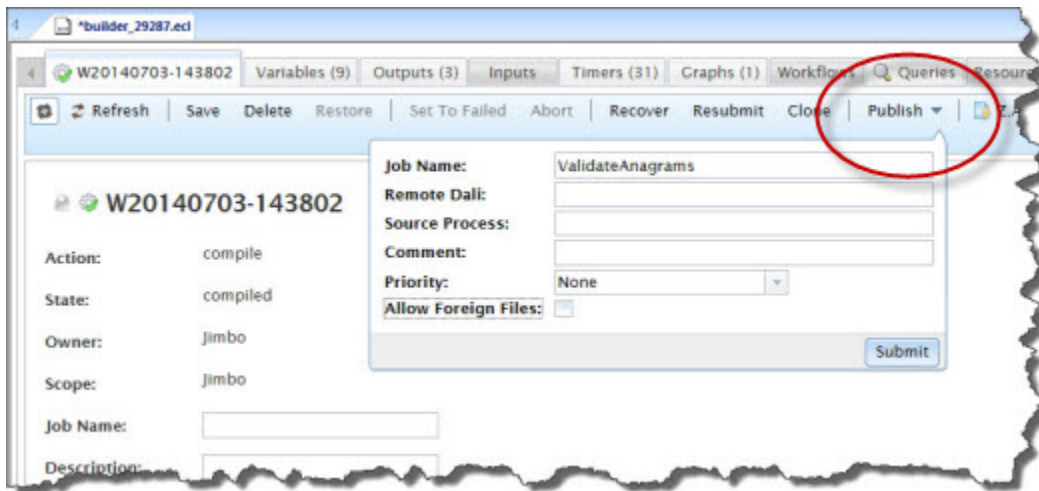
Figure 29. Publish Query
