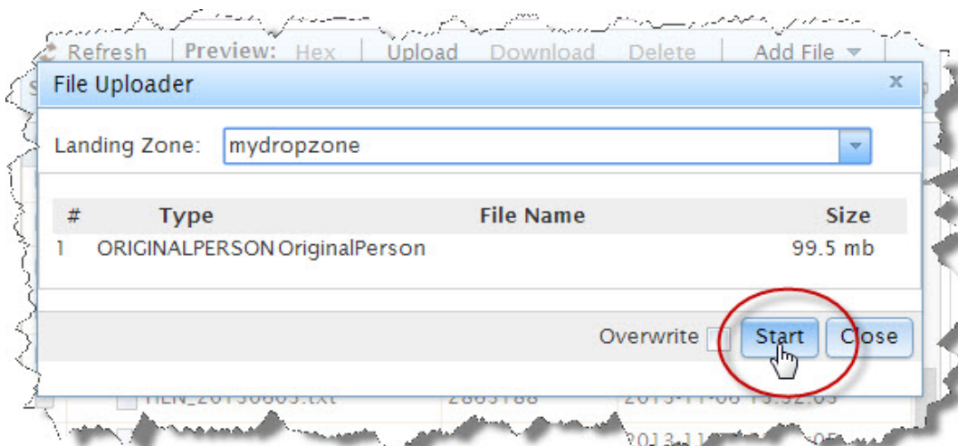
Figure 33. Dropzones
