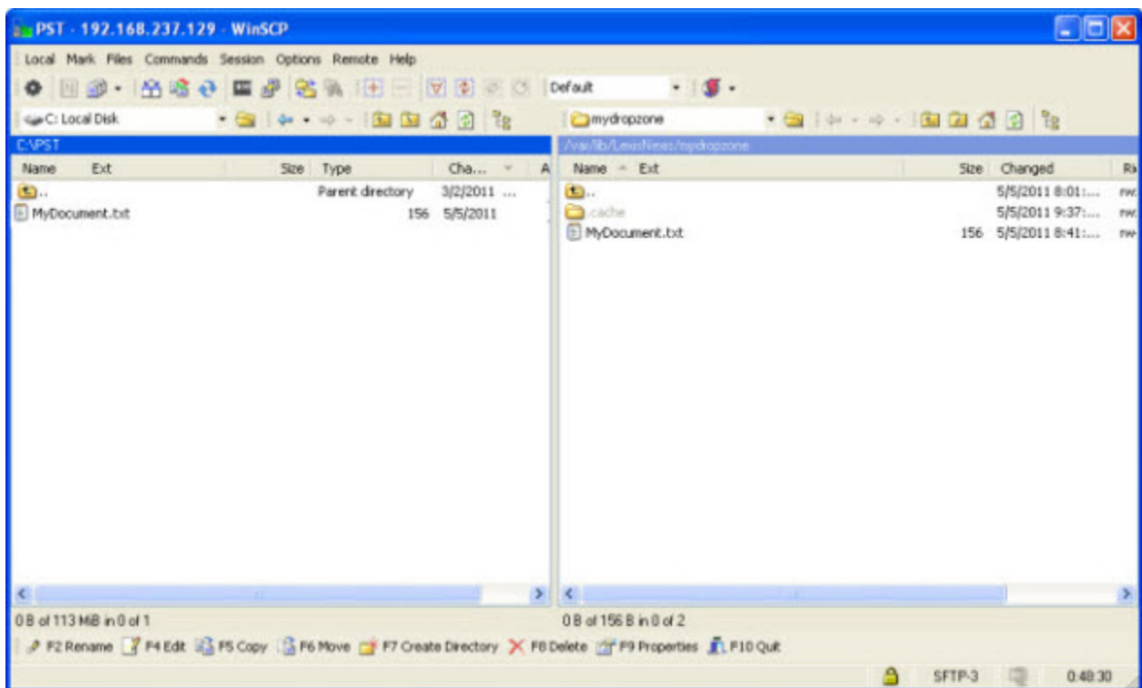
Figure 34. WinSCP
