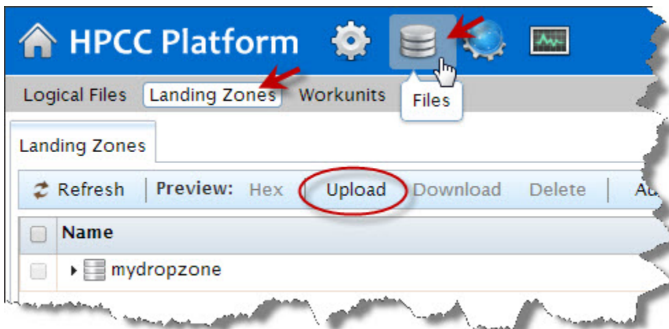
Figure 21. Upload
