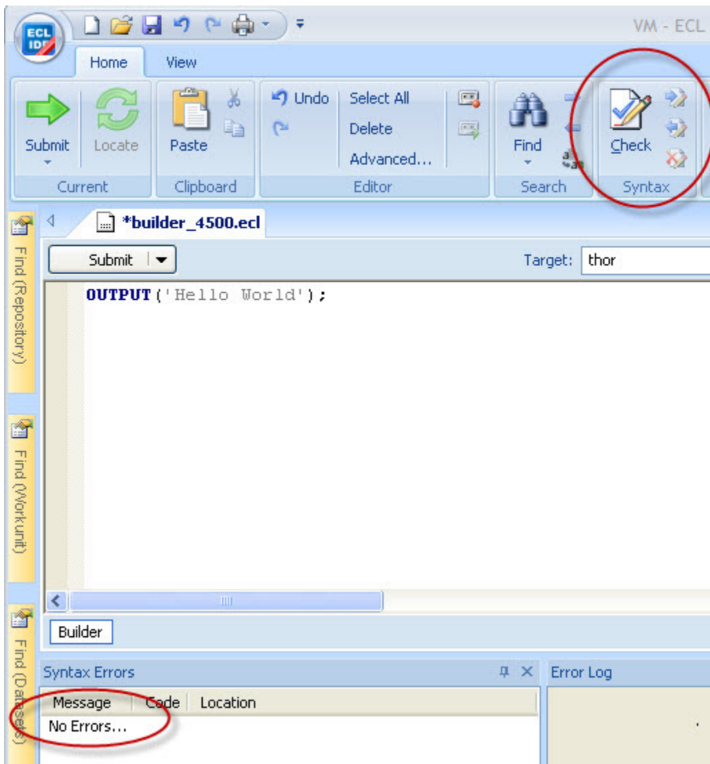
Figure 17. Syntax Check
