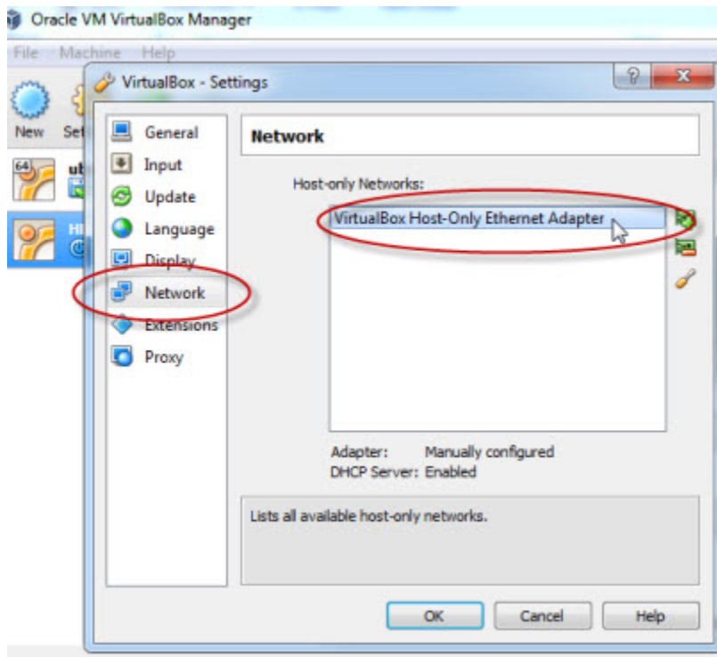
Figure 3. VirtualBox - Settings
