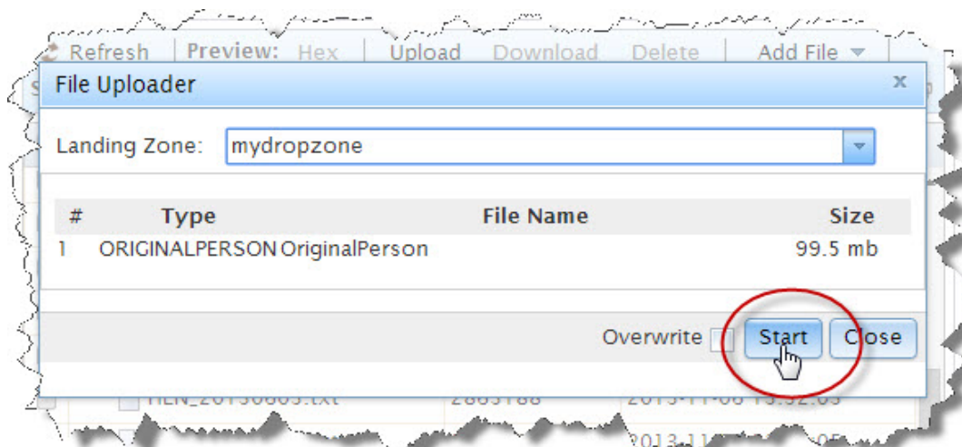
Figure 34. Dropzones
