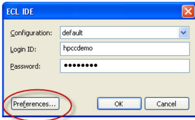
Figure 12. Login Window
