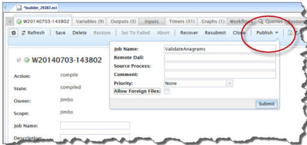
Figure 30. Publish Query
