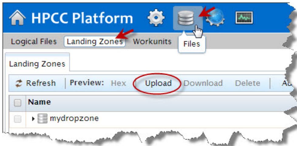
Figure 33. Upload/download
