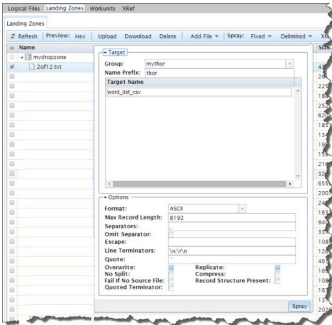
Figure 24. Spray Delimited
