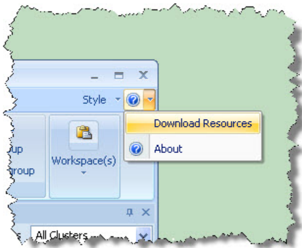
Figure 37. Help Menu
