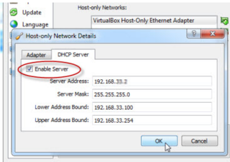
Figure 4. Network Details
