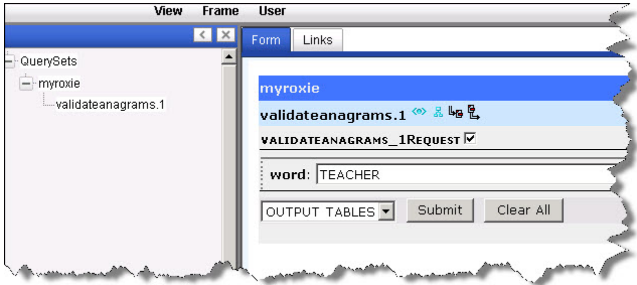
Figure 31. RoxieECL
