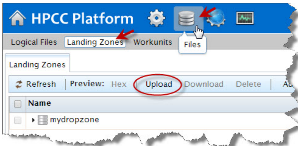
Figure 22. Upload
