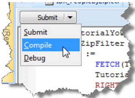
Figure 22. Compile
