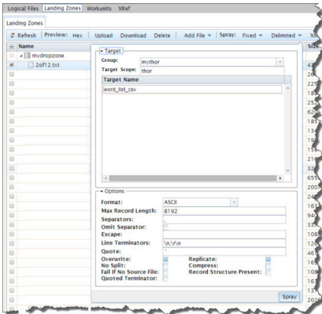
Figure 18. Spray Delimited
