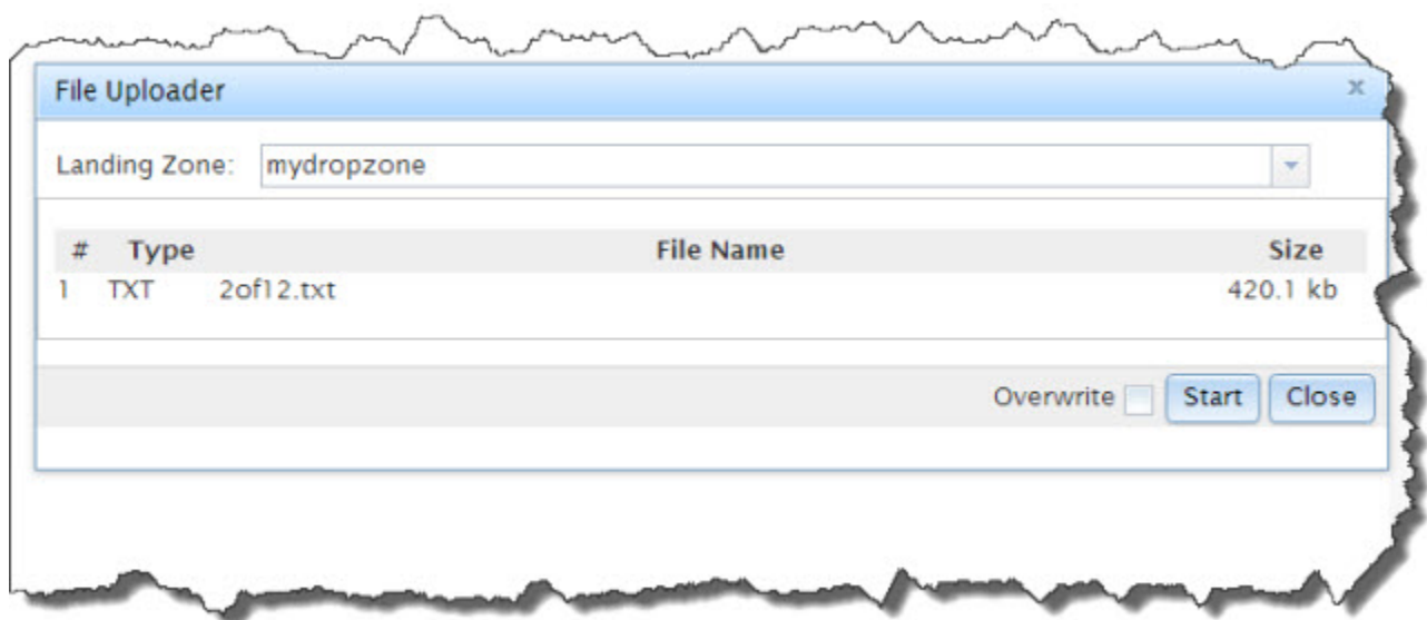
Figure 17. File Uploader
