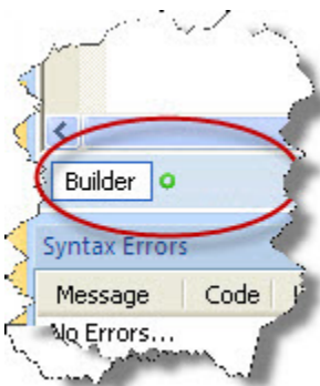
Figure 23. Compiled
