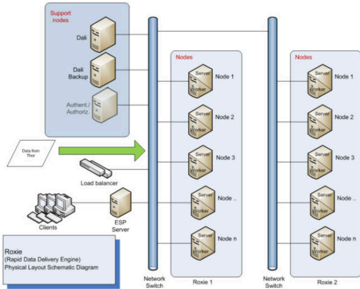
Figure 2. System Overview: Roxie
