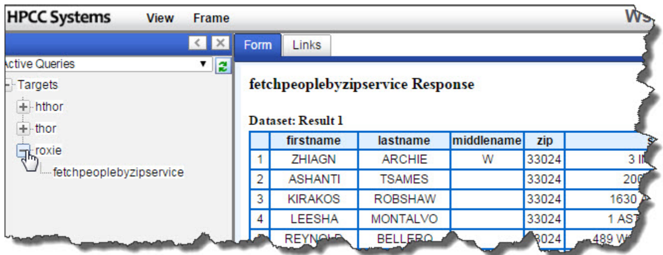
Figure 30. RoxieResults
