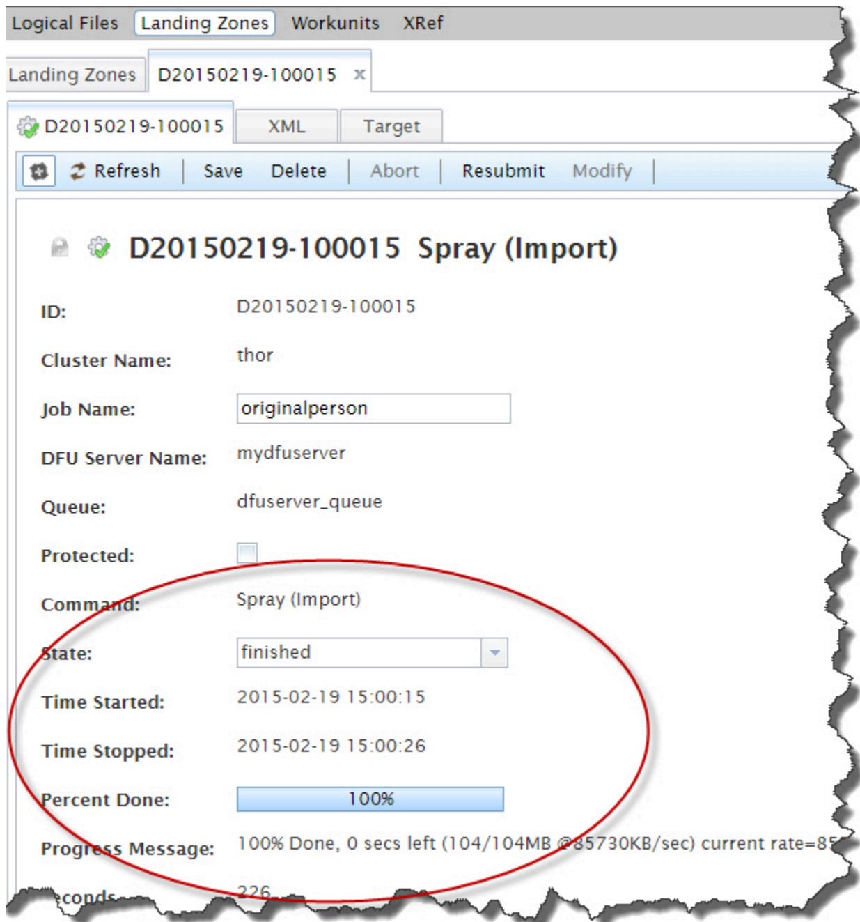
Figure 7. View Progress
