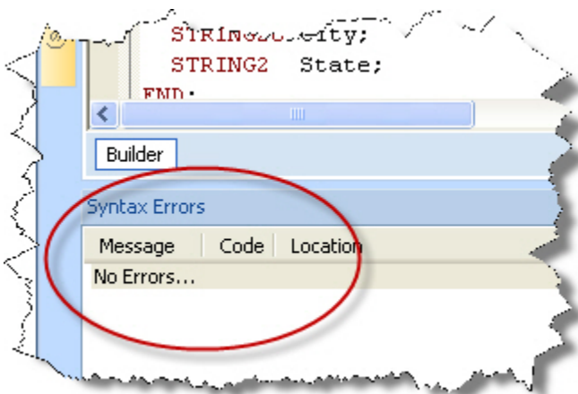
Figure 13. Check Syntax
