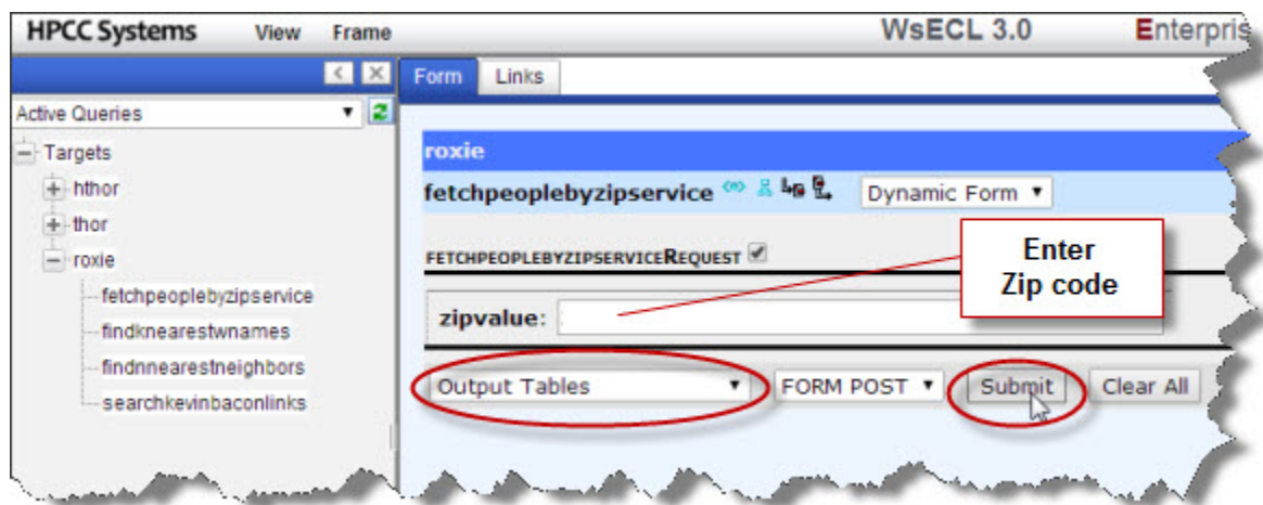
Figure 29. RoxieECL
