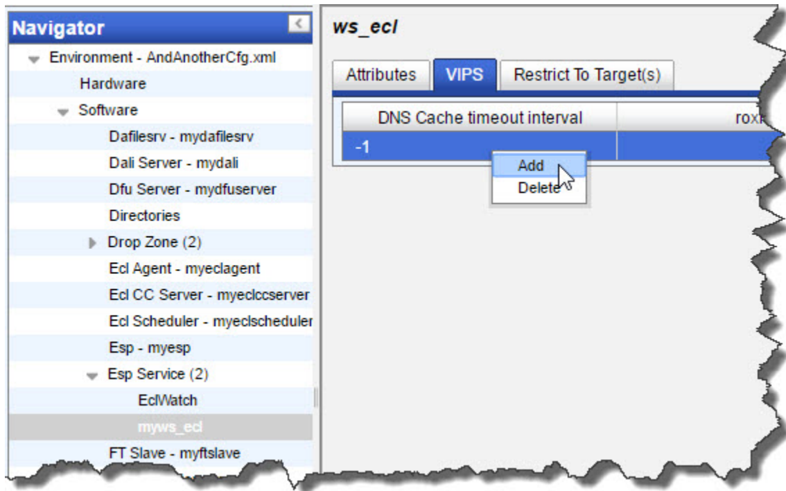
Figure 30. Configure VIP
