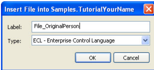
Figure 14. Insert File
