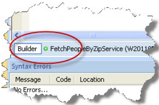
Figure 27. Compiled
