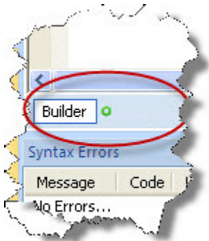
Figure 24. Compiled
