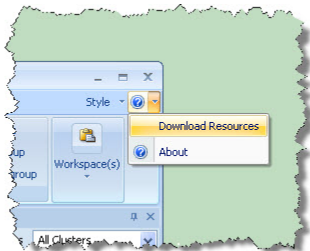
Figure 28. Help Menu
