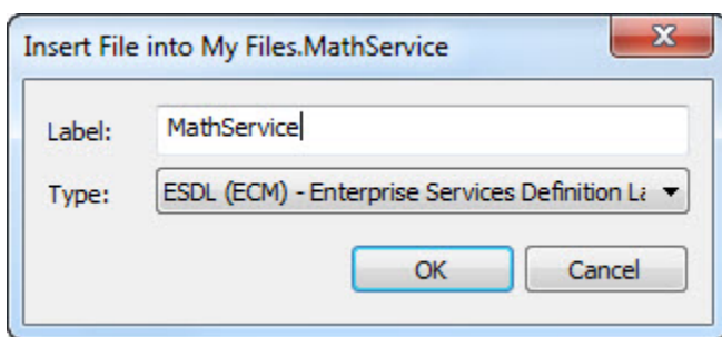
Figure 3. Insert File
