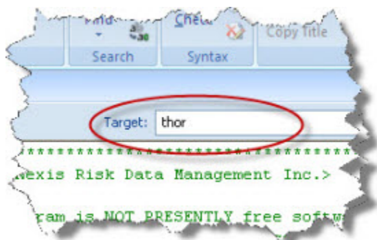
Figure 36. Target: thor
