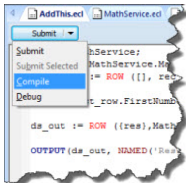
Figure 8. Compile
