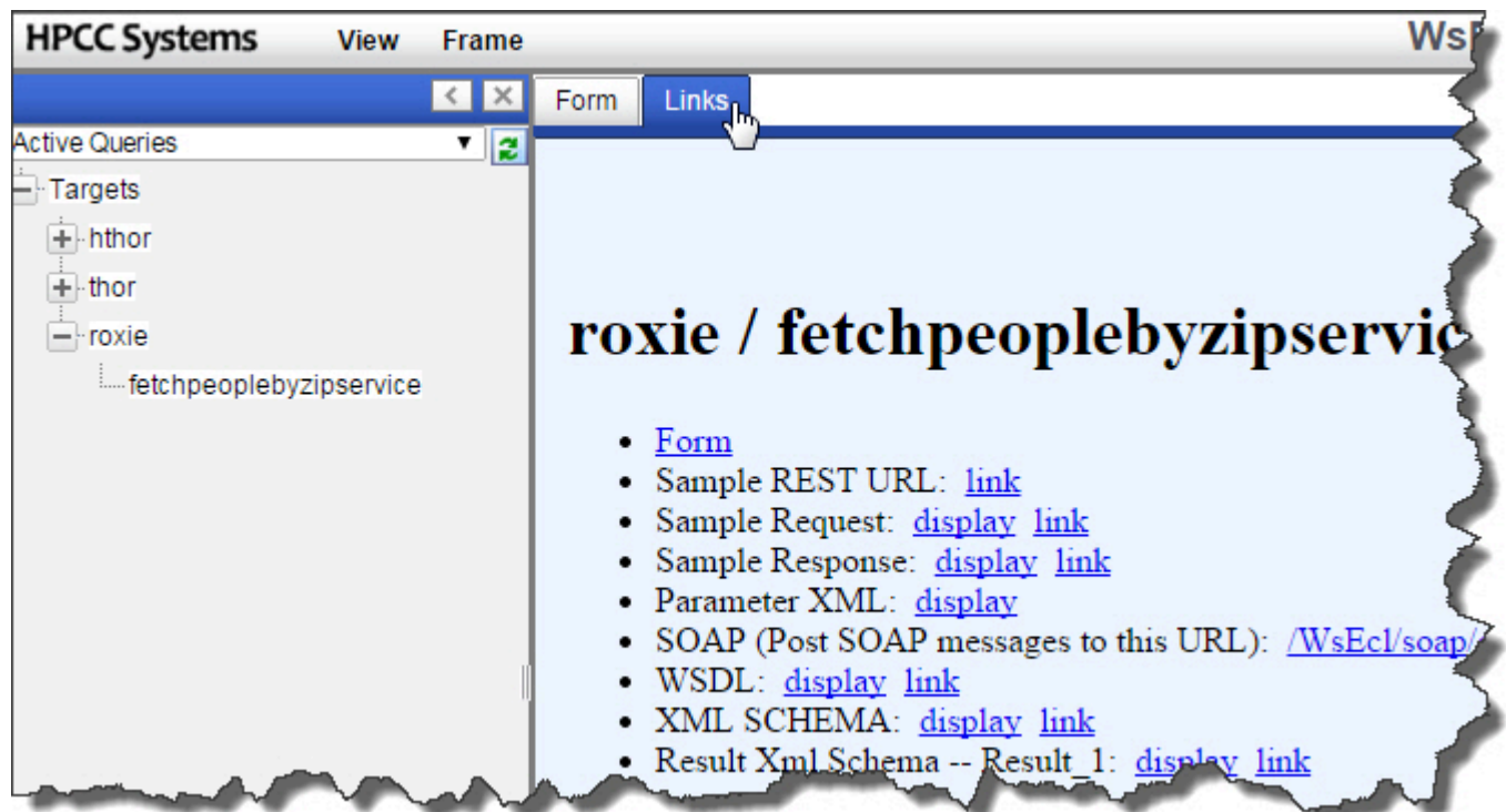
Figure 31. Links
