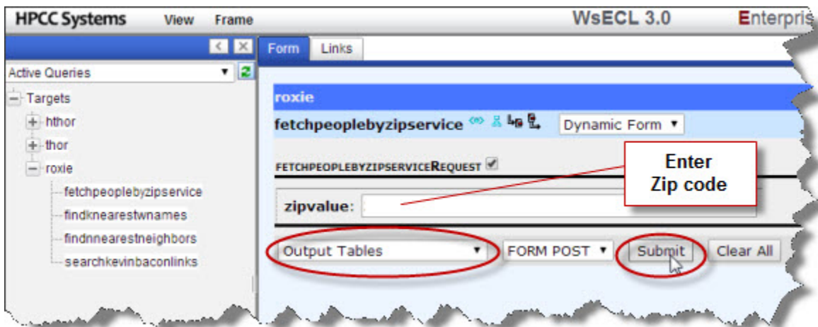
Figure 29. RoxieECL
