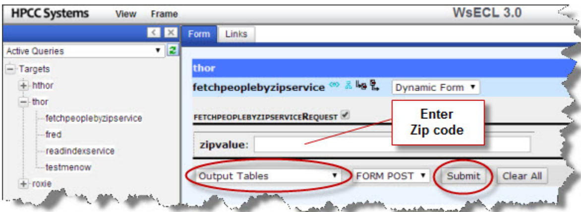
Figure 23. Service Form
